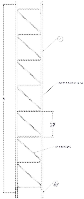
ELEVATION VIEW
