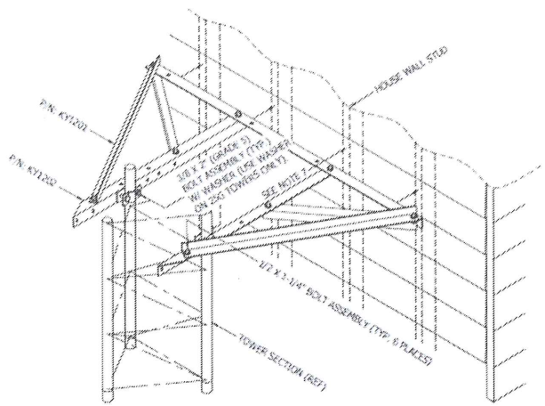
HOUSE BRACKET DETAILS (ORDER ASSEMBLY PART NO. H5UTVRO)
