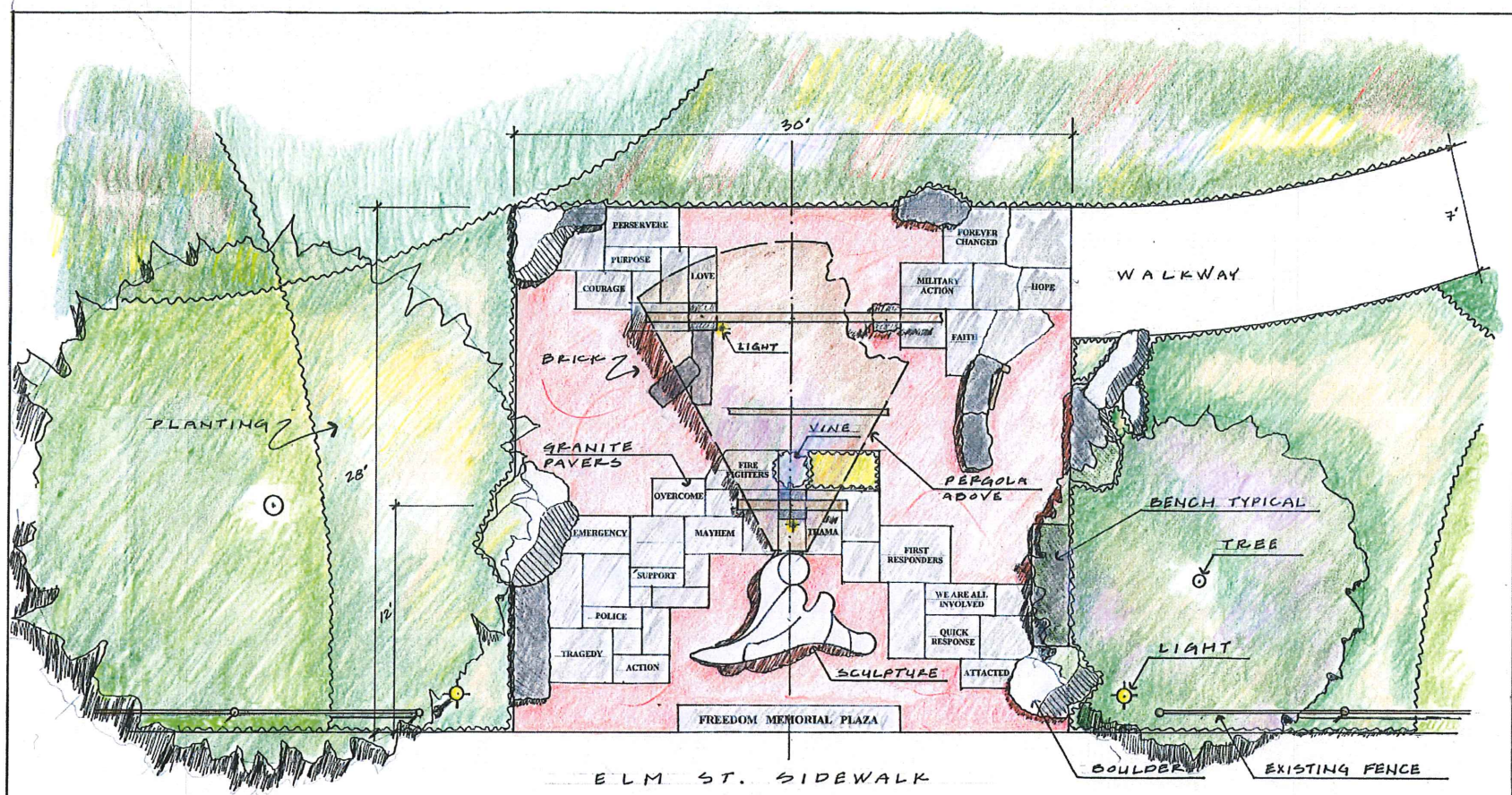
1 L-1 FREEDOM MEMORIAL SITE PLAN SCALE: 1/4" = 1'-0"
